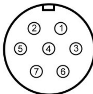
2PMГ18Б7Ш1Е2 male connector 2PMГ18Б7Ш1Е2 вилка
