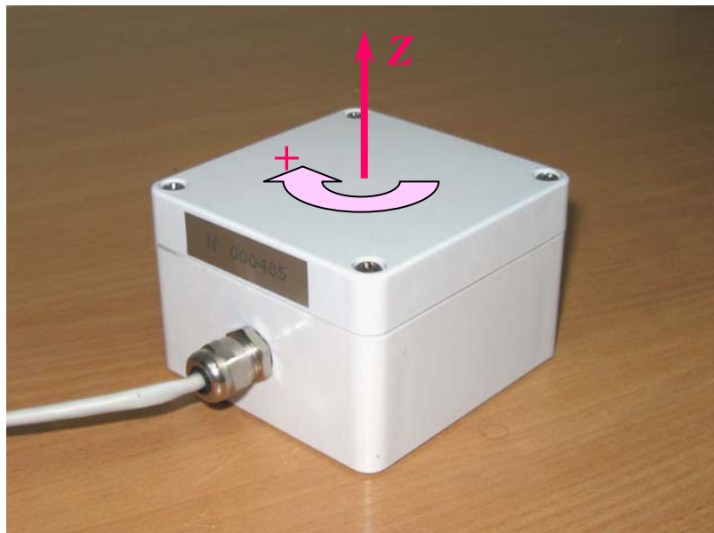
Fig. 1. Direction of the rotational sensing axis of the seismic sensor METR-01.
