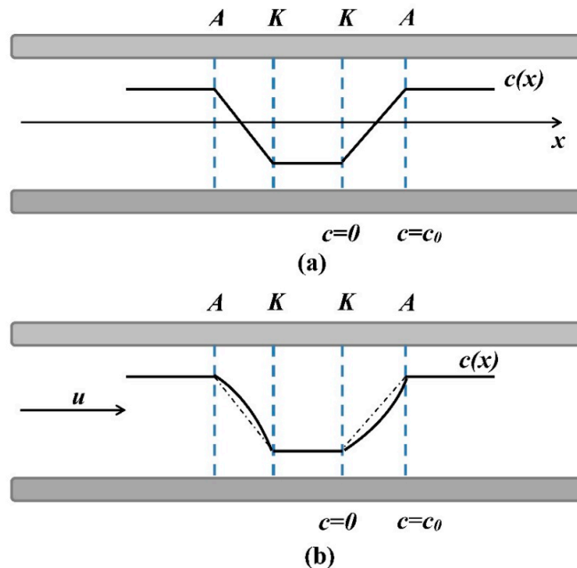
Figure 2. The carrier concentration gradient in the transducing cell under the influence of external pressure variations. c(x) is the ion concentration; (a) distribution without external pressure variations; (b) the distribution of concentration c(x) varies under the oncoming flow of liquid; u = fluid flow rate. A = anode, K = cathode.
