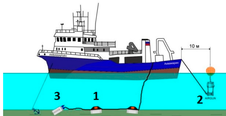
Figure 7. The scheme of the marine test. (1) hydrophones to compare; (2) single pneumatic source; (3) remote acquisition module.
