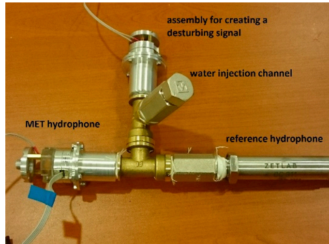
Figure 3. The hydraulic bench.
