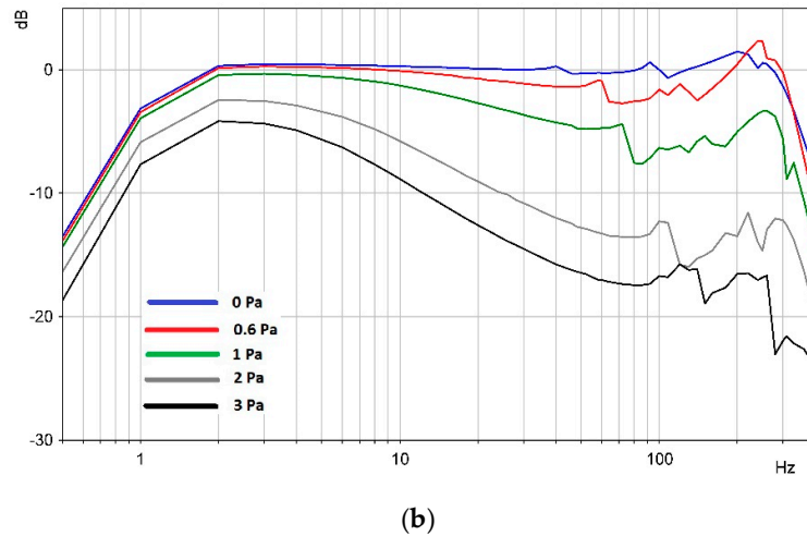
Figure 4. Frequency response curves (0.8 mV/Pa) of the MET hydrophones under different pressure differences. (a) With the volume completely filled with liquid under the upper cover; (b) with the partially filled volume.
