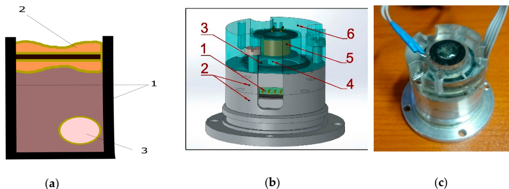
Figure 1. Hydrophone: (a) scheme; (b) design [19]; (c) experimental sample [19].
