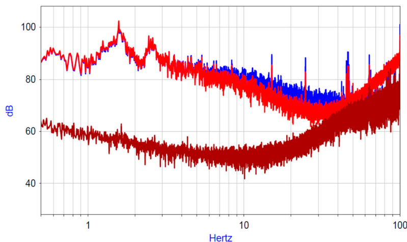
Figure 5. Power spectral density of the hydrophone signals. Blue and light-red lines are the spectra of the hydrophone signals. Red line is the noise spectral density.
