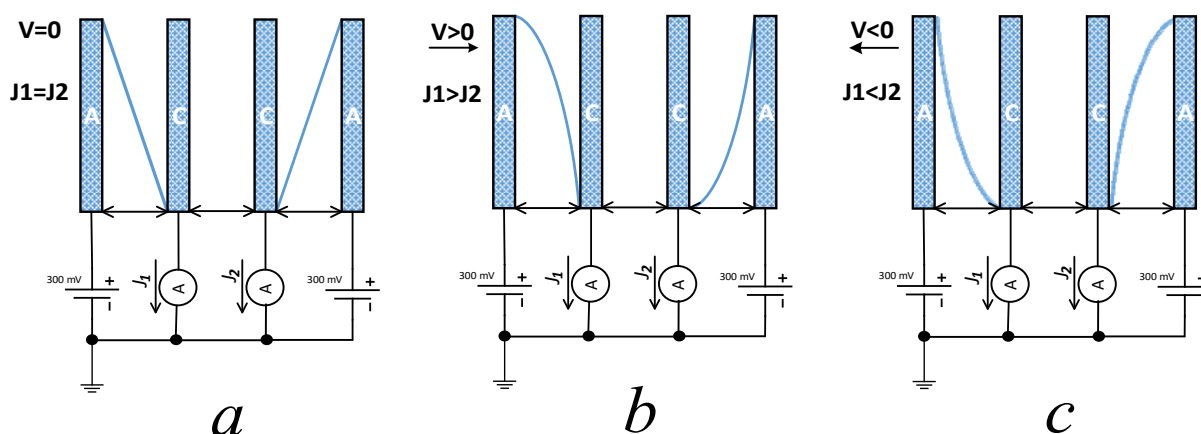
Figure 2. The distribution of active component concentration in electrolyte. (a – steady state, b and c moving to the right and left respectively).
