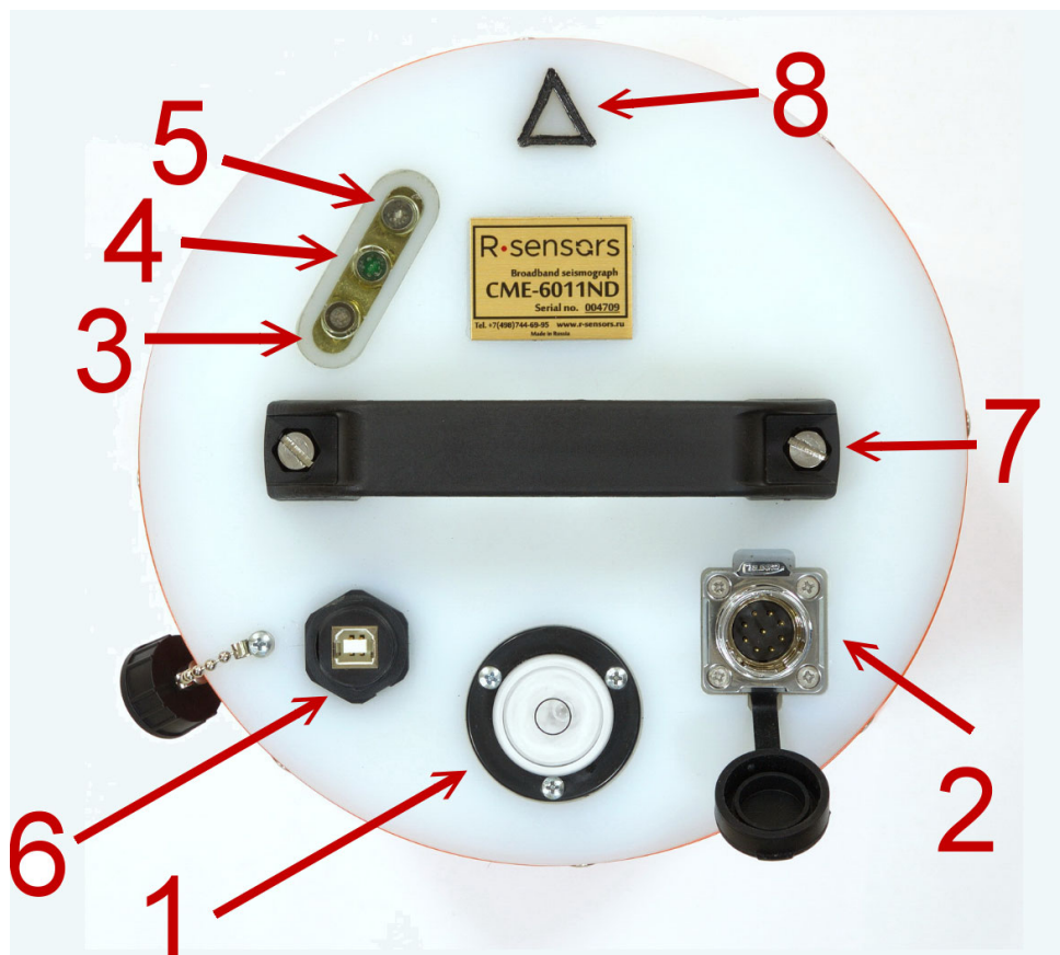
Fig. 1. Connectors and Indicators
