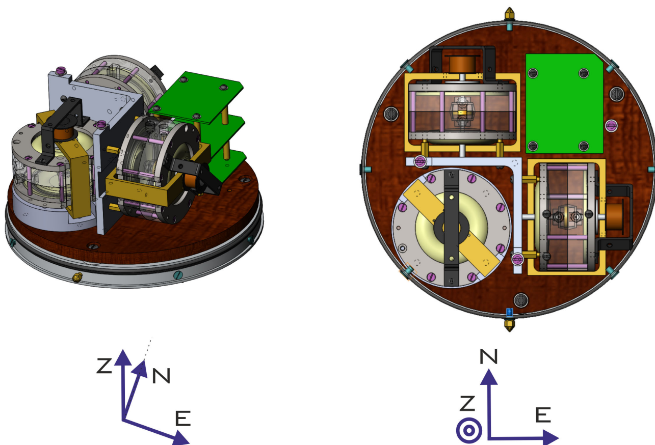
Fig.1 The transducers' geometrical configuration of CME-6011ND.
