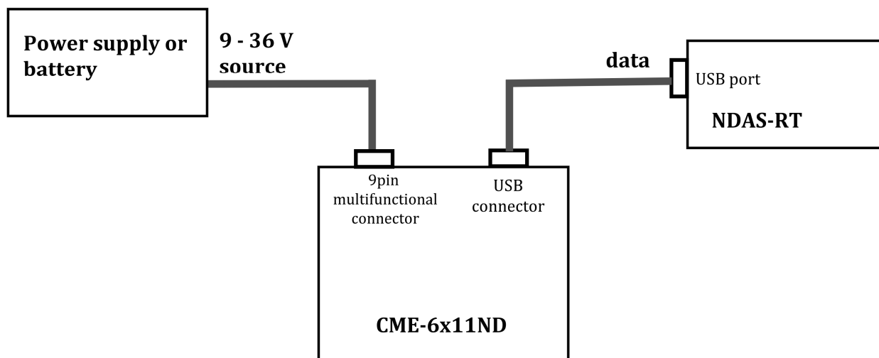
Fig. 3. Power supply from the power supply, data transfer to NDAS-RT via the USB port. (main operating mode, SD card reading mode)
