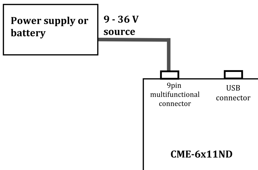
Fig. 1. Power supply from the power supply (main operating mode)
