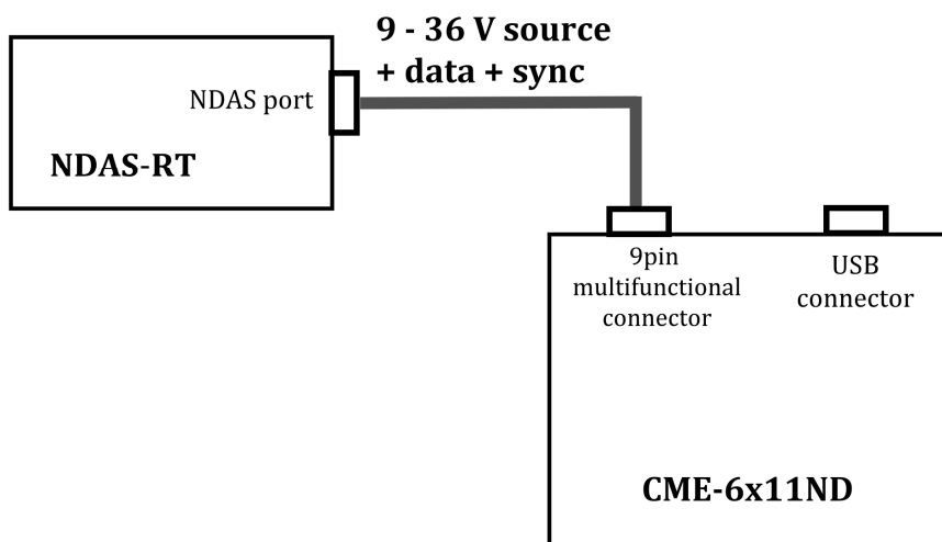
Fig. 2. Working with NDAS-RT. Power supply, data transfer and synchronization via cable through NDAS-port (main operating mode)
