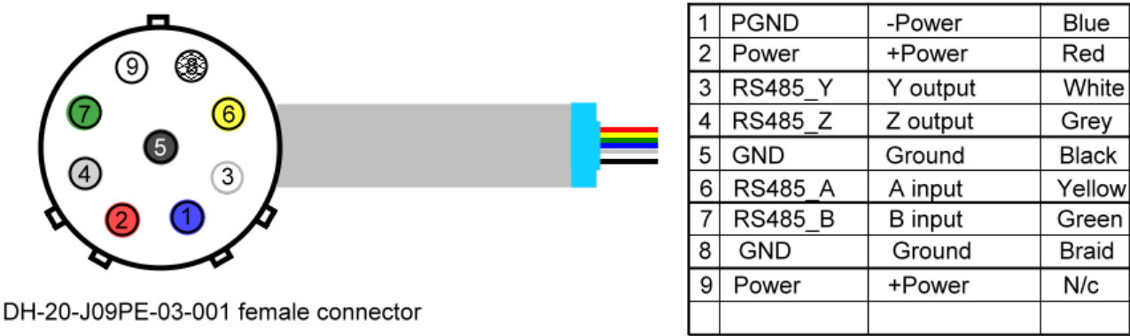
Fig. 1. Multifunctional connector, combined cable
