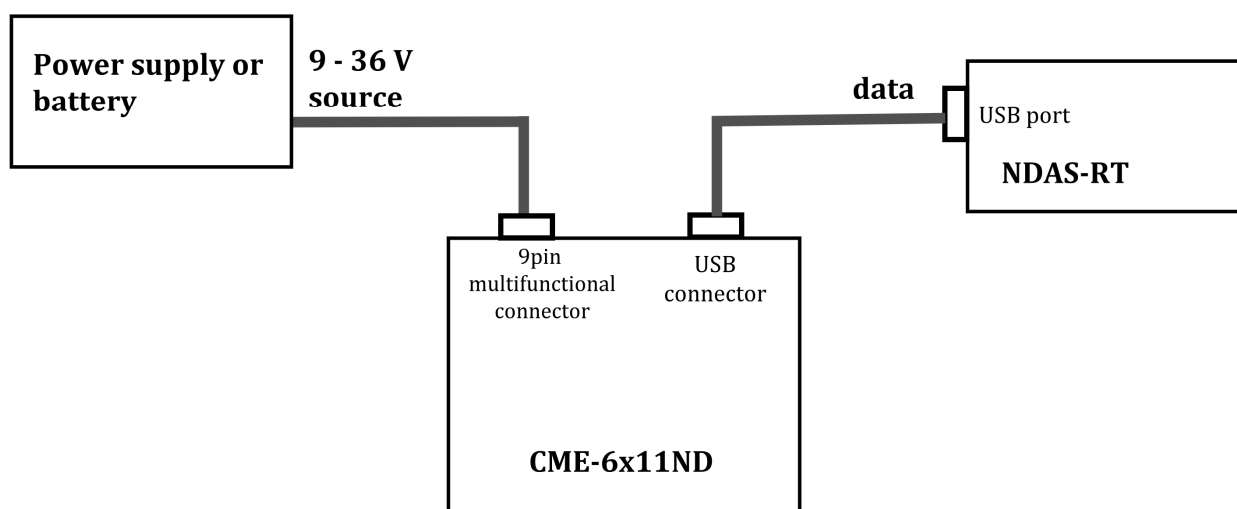
Fig. 4. Power supply from the power supply, data transfer to the computer. (main operating mode, SD card reading mode). When connected only via USB (without a power supply), only setup and reading of saved data is possible.
