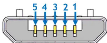
Pinout of Micro B
